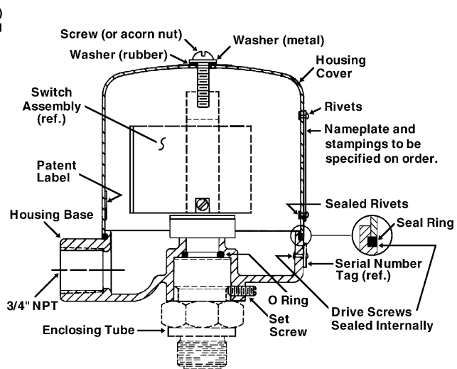
Carbon Steel Housing Assembly Figure 6
