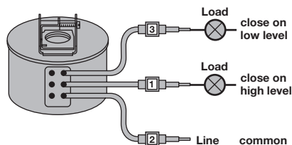
Figure 8 SPDT Terminals for Series HS only
