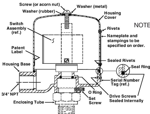
Figure 16 Carbon Steel Housing Assembly
