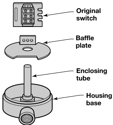
Figure 10 Original Switch Configuration
