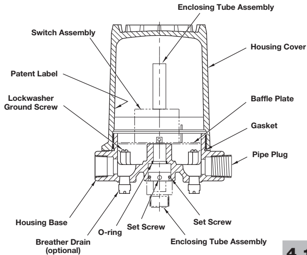
Figure 14 Aluminum Housing Assembly
