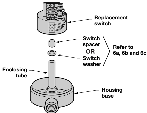
Figure 11 Replacement Switch
