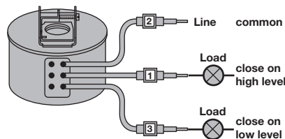
Figure 7 SPDT Terminals for Series H1 only
