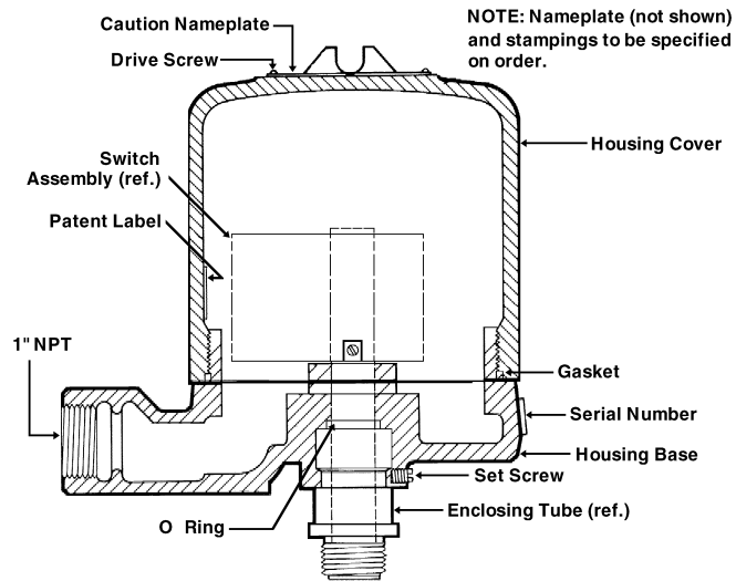
Figure 15 Cast Iron Housing Assembly
