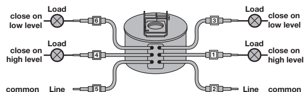
Figure 9 DPDT Terminals for Series HS only
