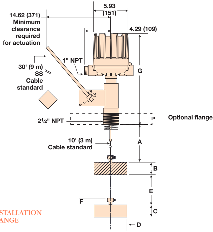
HOLLOW BRASS DISPLACER
