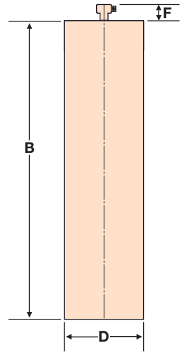
HOLLOW BRASS DISPLACER
