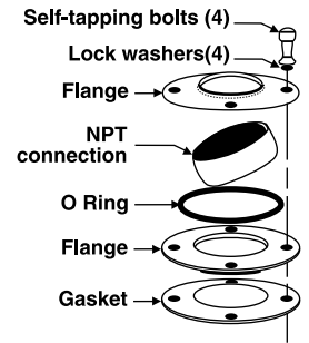
VERSA FLANGE ASSEMBLY PART NUMBER 089-5207-001
