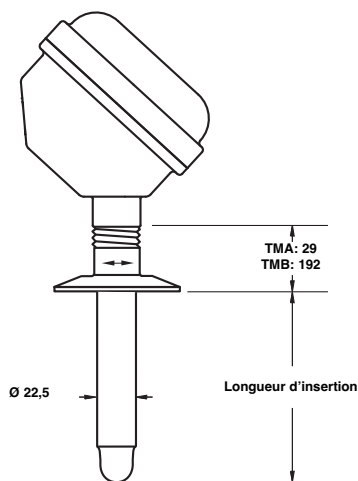
Tri-Clamp®
