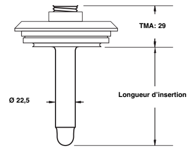
Varivent®
