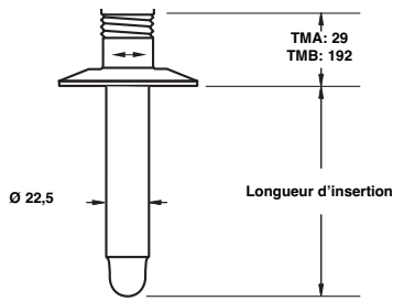
Tri-Clamp®
